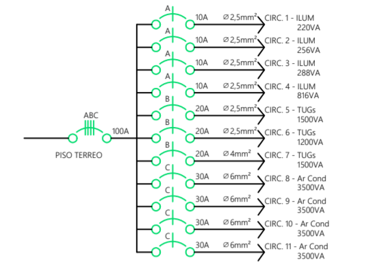
03 DIAGRAMA UNIFILAR GERAL
